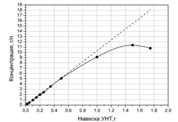
Solubility dependence of modified CNT and initial CNT in water solution
