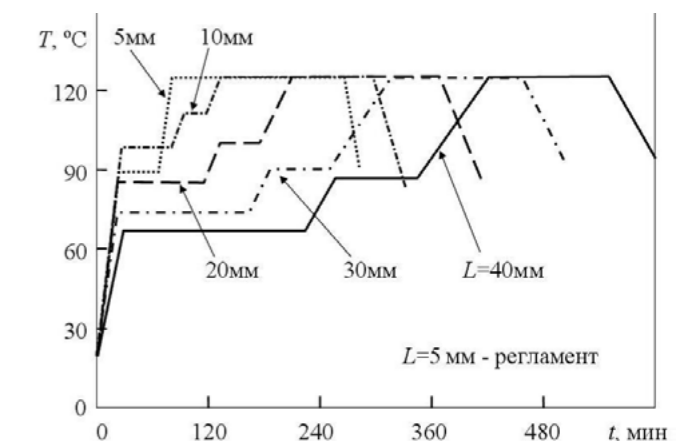
Optimal curing modes for fiberglass panels of different thicknesses
