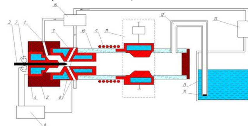
1 – hole in dielectric frame; 2 – dielectric frame; 3 – cathode; 4 – cathode holder; 5 – anode; 6 – device for cathode automatic movement; 7 – rolls; 8 – powder supply port; 9 – inductor; 10 – operating camera; 11 – high-frequency generator; 12 – output tube; 13 – reservoir; 14 – net; 15 – pneumatic pump; 16 – gas-carrier distributor.
