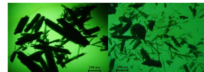
Ultrafine powder of manganese oxide before (left) and after plasma torch treatment
