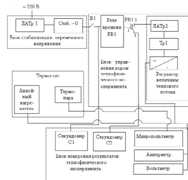
Functional scheme
