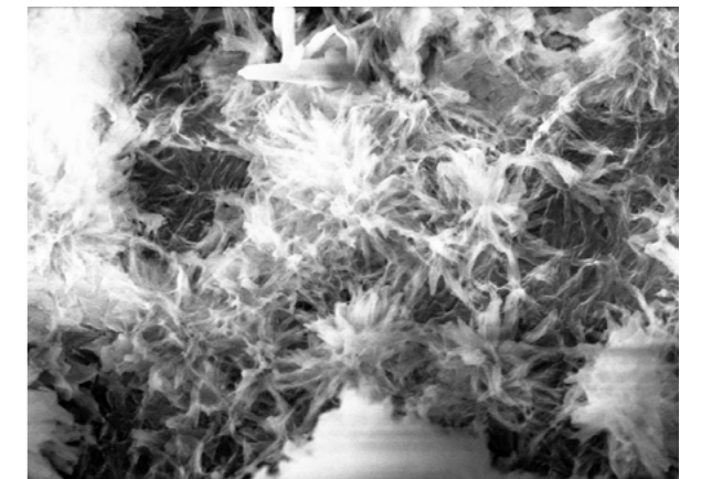
Electron microphotos of unmodified structure (top) and of nanomodified grained concrete
